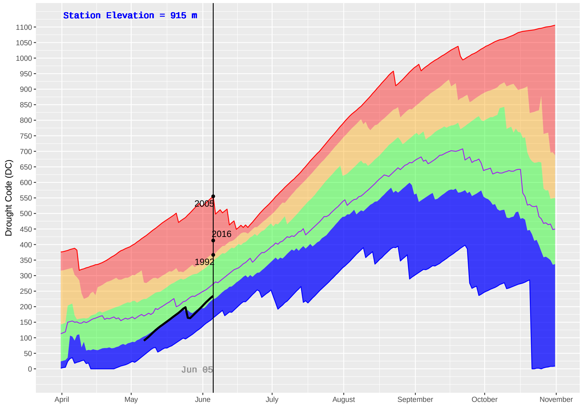
MIDDLE LAKE (226) : Historical (1989–2018) and Current (2019) Daily Drought Code (DC)
