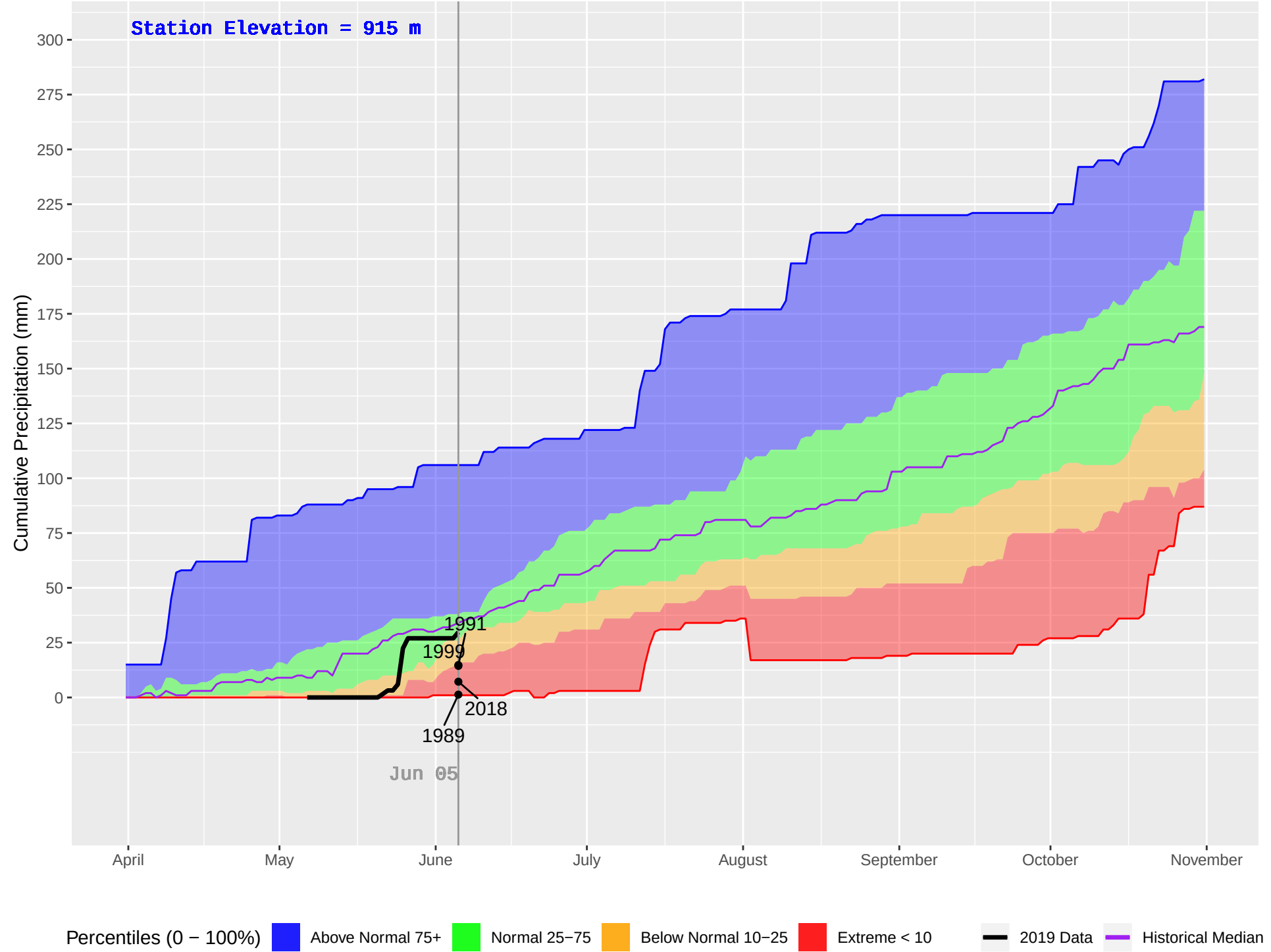
MIDDLE LAKE (226) : Historical (1989–2018), Current (2019) Daily Cumulative Precipitation
