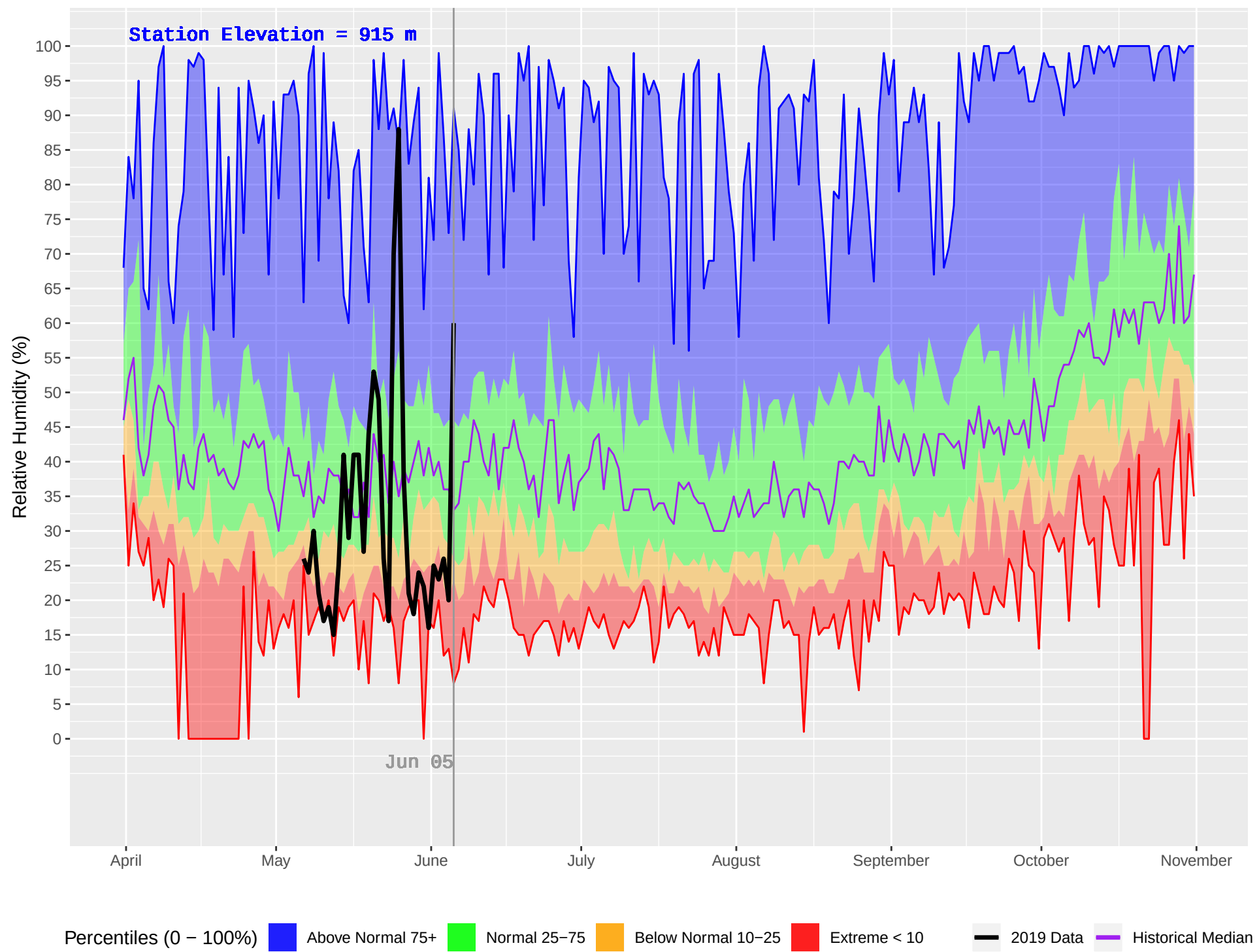
MIDDLE LAKE (226) : Historical (1989–2018) and Current (2019) Daily Relative Humidity
