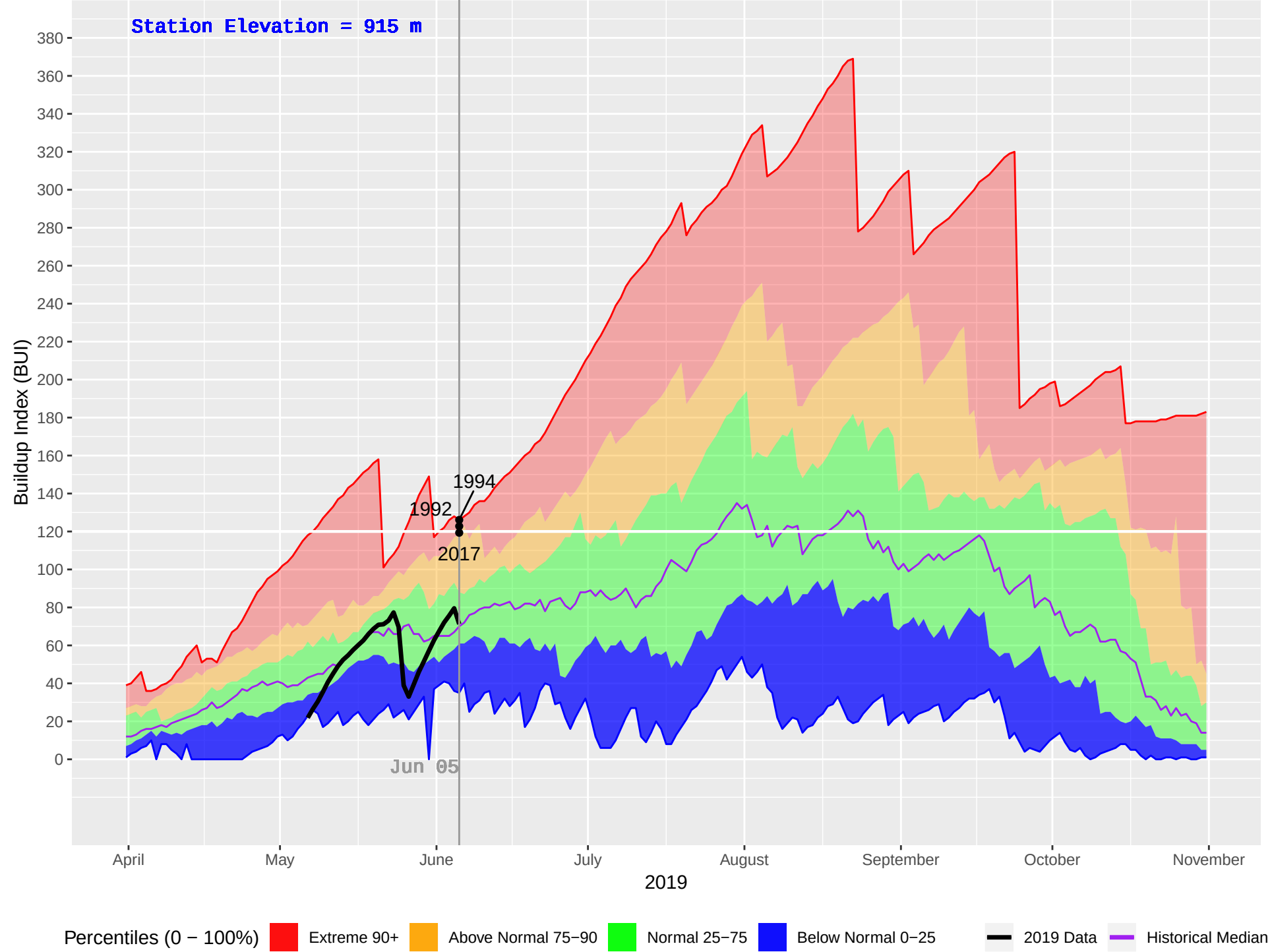
MIDDLE LAKE (226) : Historical (1989–2018), Current (2019) Daily Buildup Index (BUI)
