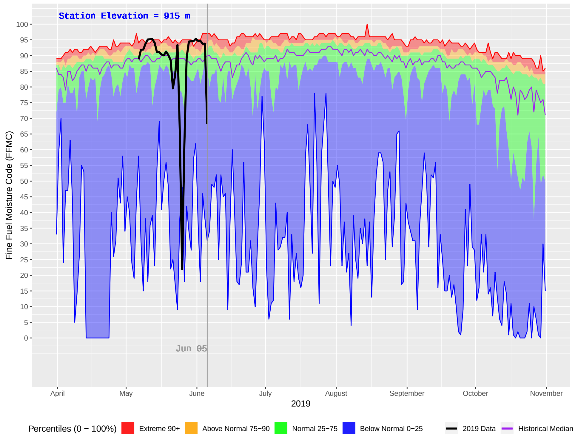
MIDDLE LAKE (226) : Historical (1989–2018) and Current (2019) Daily Fine Fuel Moisture Code (FFMC)
