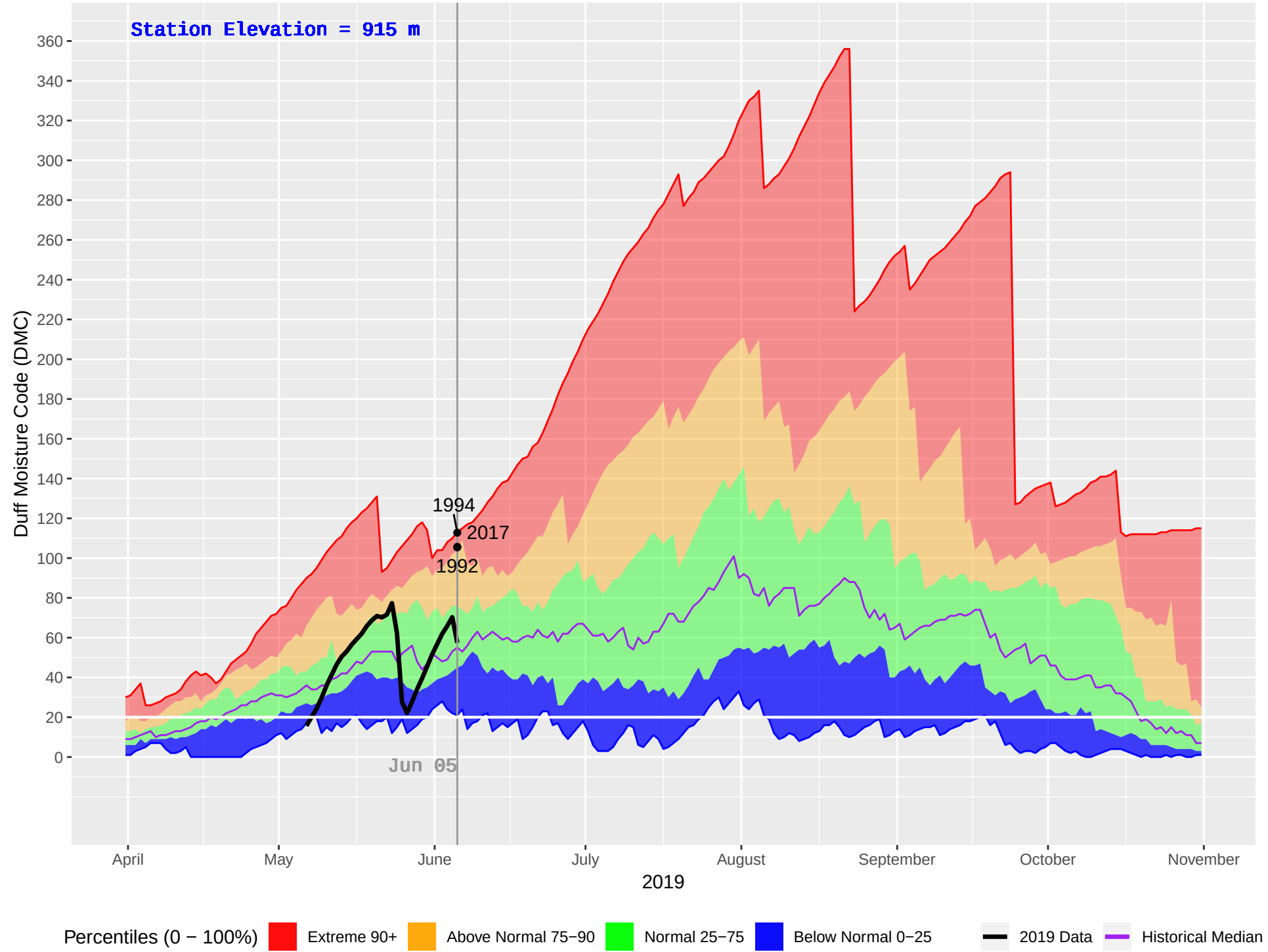
MIDDLE LAKE (226) : Historical (1989–2018), Current (2019) Daily Duff Moisture Code (DMC)
